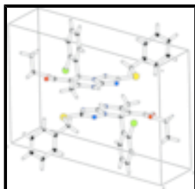
Fig. 2. A packing diagram of (I).
